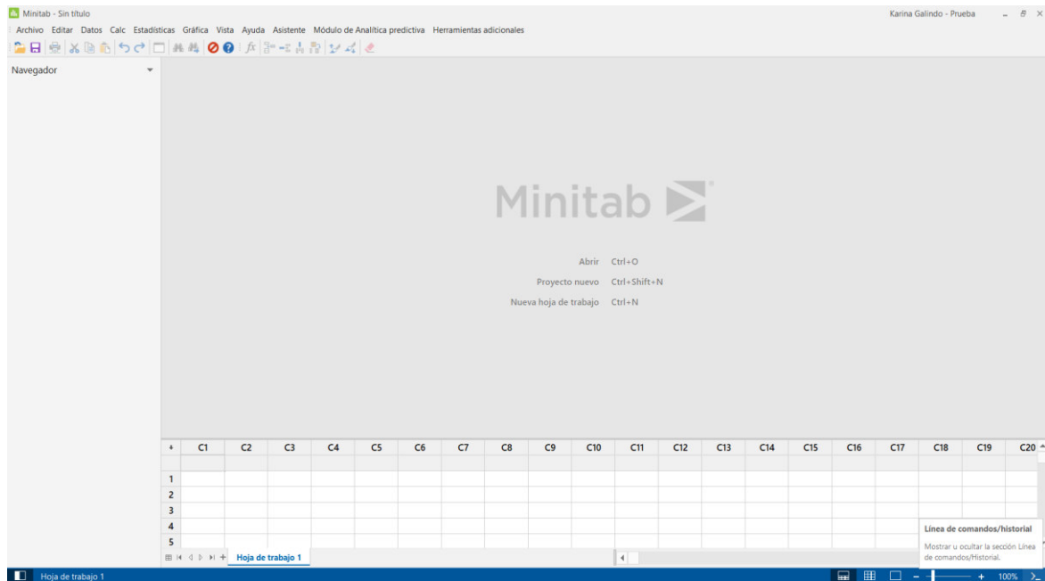
Figura 49. Software Minitab
