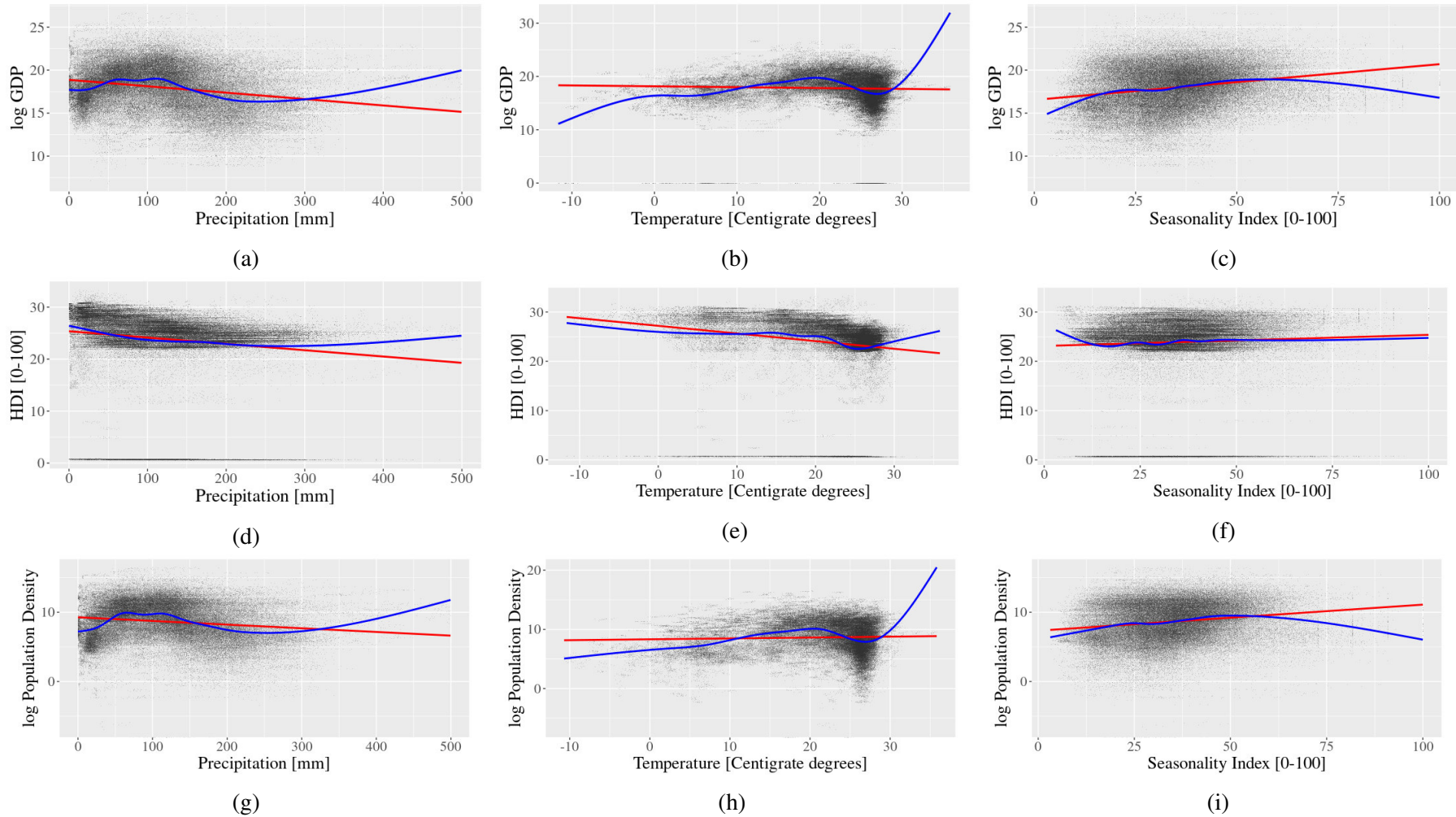
Figure 2: Scatterplots at the grid cell level
