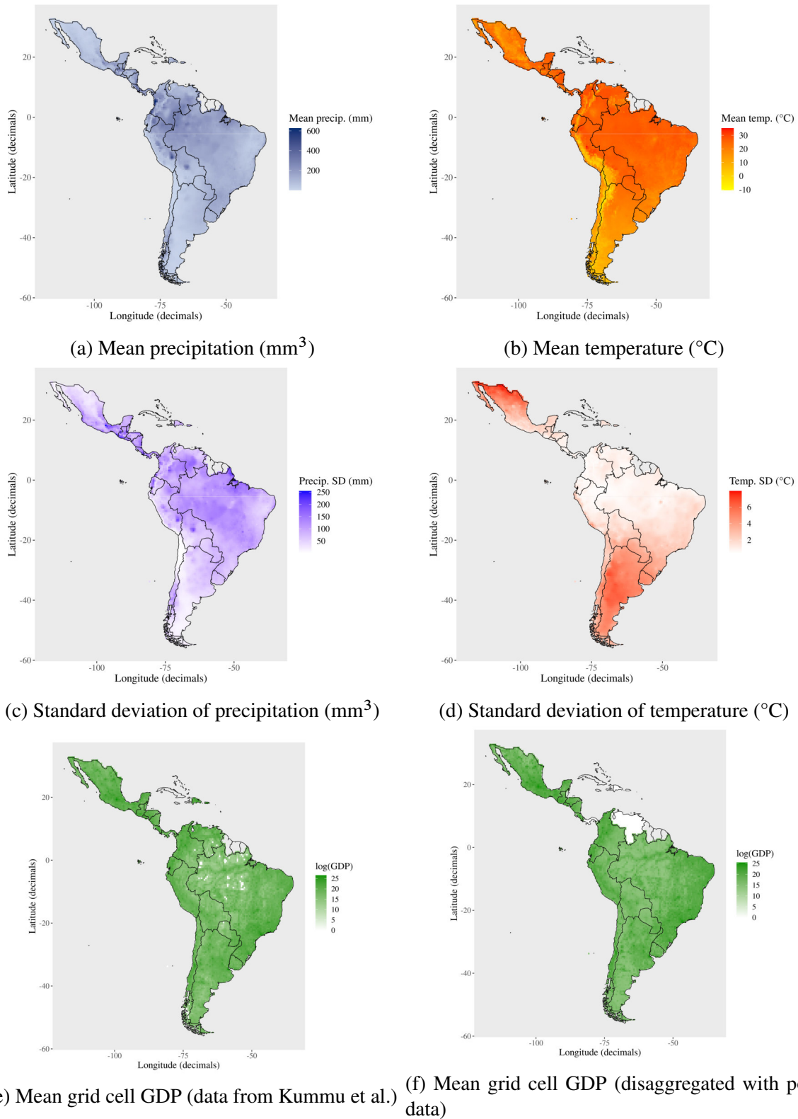
Figure 1: Spatial distribution of variables
