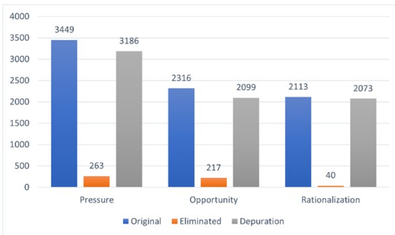
Figure 4.6: Vertex FraudTriangle_Stages.
