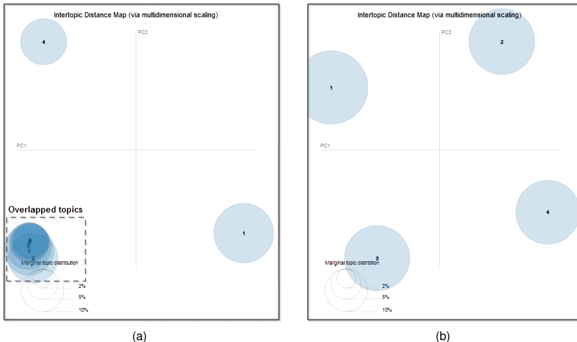
Figure 3.5: Intertopic distance map for k = 9 and k = 4 . (a) 9 topics. (b) 4 topics.
