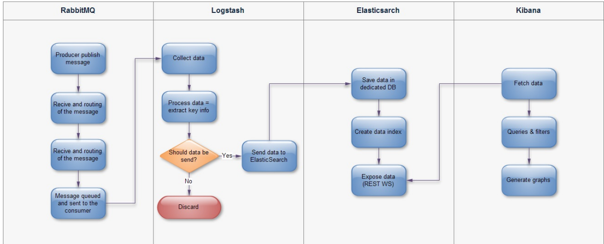
Figure A.6: Framework Implementation
